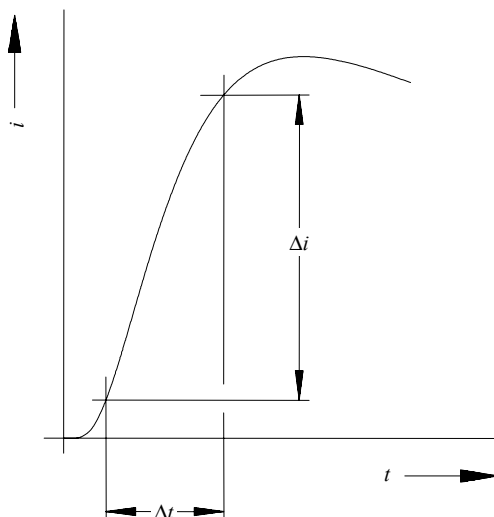
Figure C.2 – Definition for the current steepness in accordance with Table C.3
