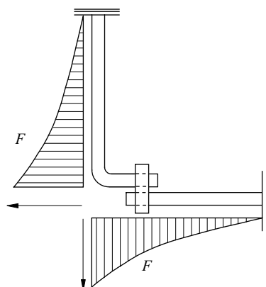
Figure D.3 – Diagram of the stresses for the configuration of Figure D.2
