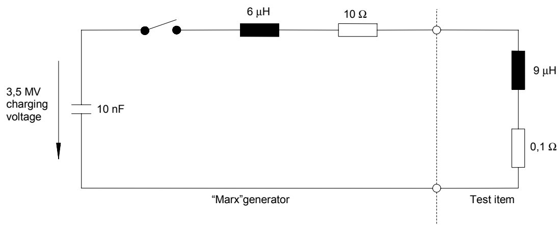
Figure C.4 – Example test generator for the simulation of the front steepness of the subsequent short strokes for large test items
