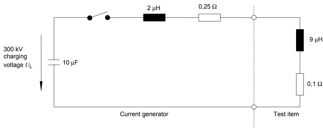
Figure C.3 – Example test generator for the simulation of the front steepness of the first short stroke for large test items
