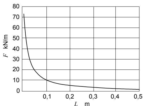
Figure D.3 – Diagram of the stresses for the configuration of Figure D.2
