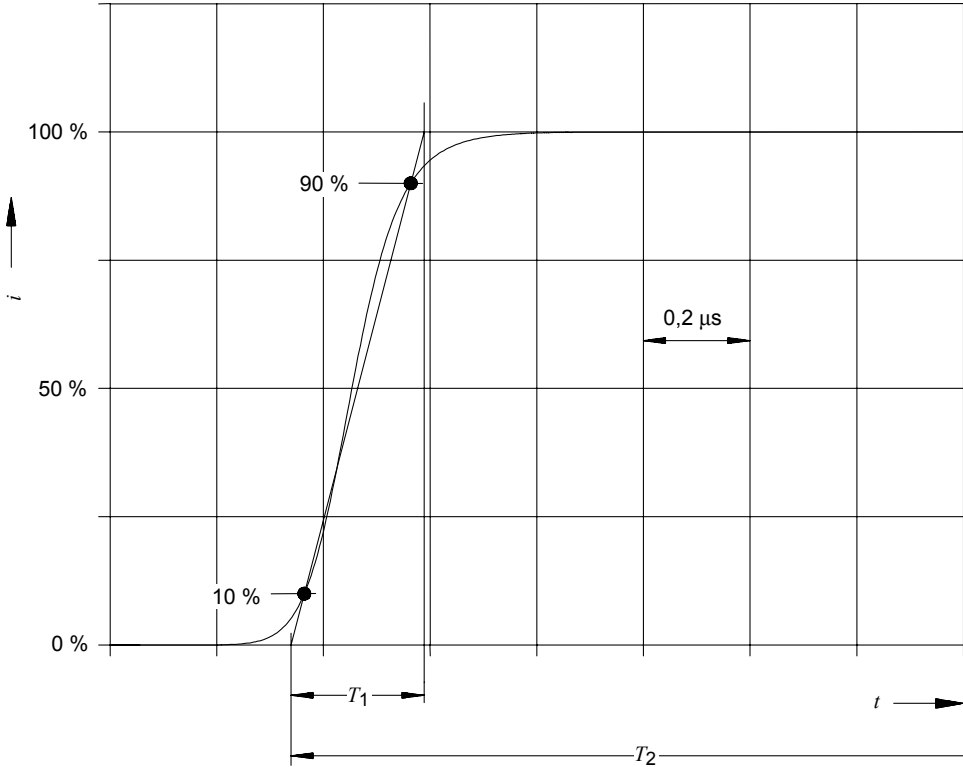
Figure B.3 – Wavelshape of the current rise of the subsequent short strokes
