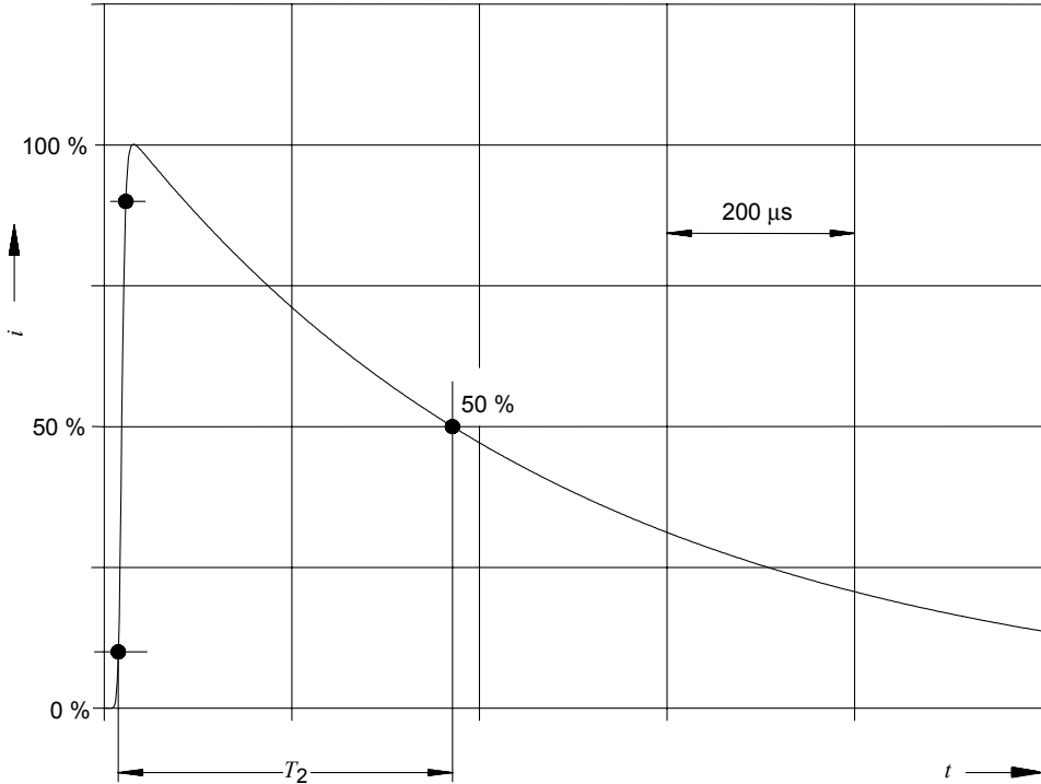
Figure B.2 – Wavelshape of the current tail of the first short stroke
